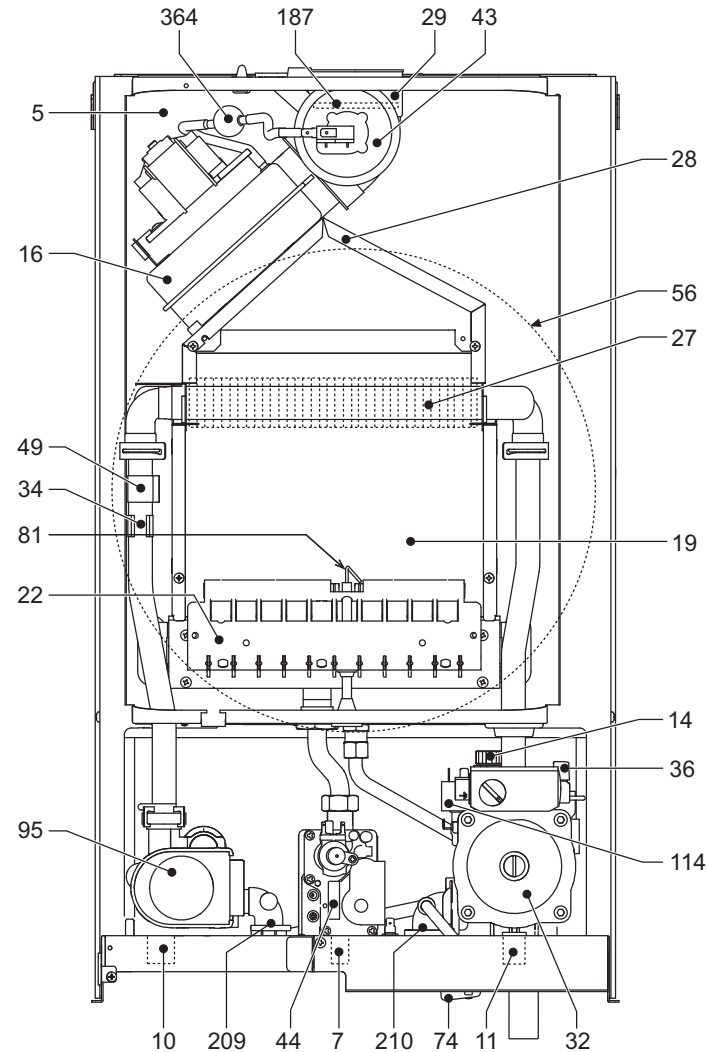
fig. 22 - Vista general
